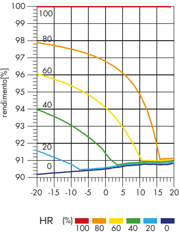
Efficiency in accordance with condensation heat
